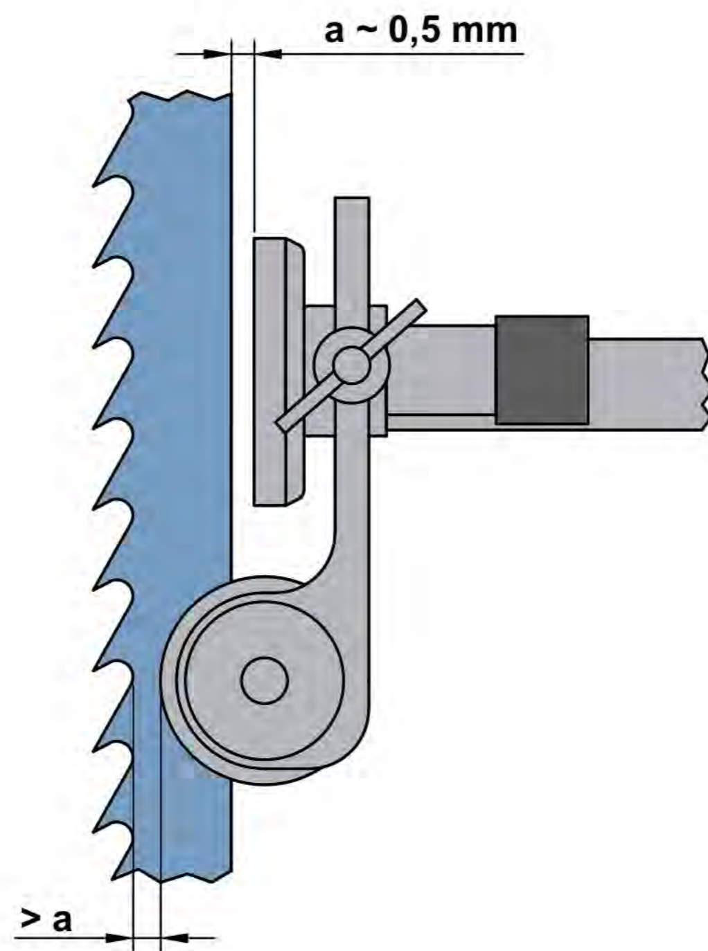
Adjustment of the saw blade guides.
