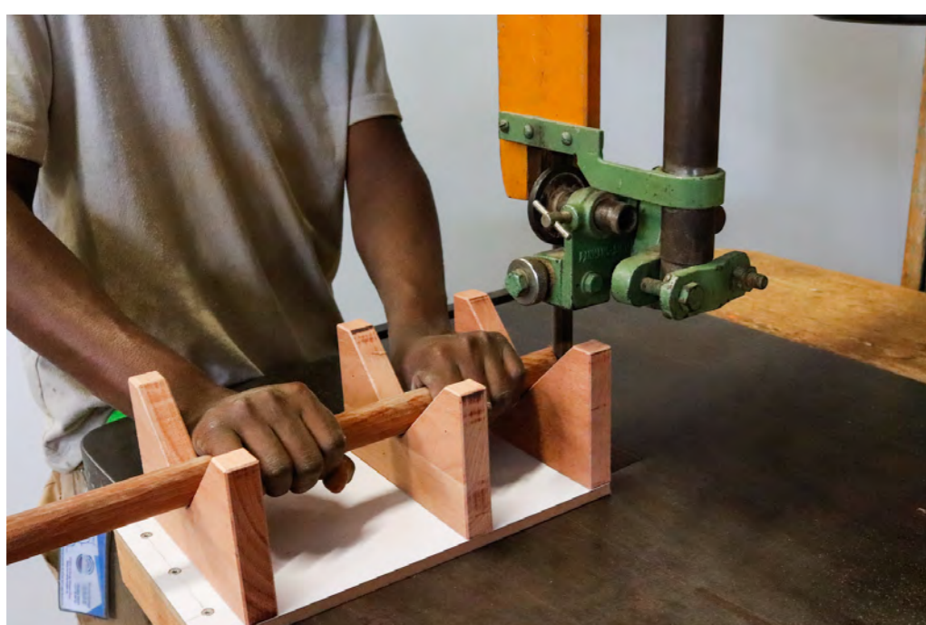
Cross cutting of round pieces with a jig.
