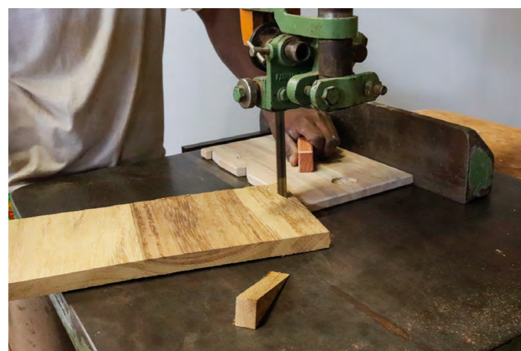
Cutting of cutter pins with a Jig.
