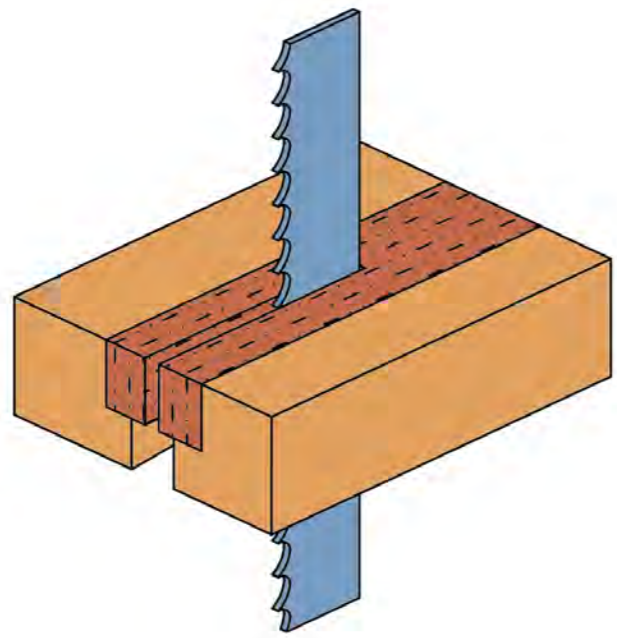
The table insert should be flush with the table, cuttable, replaceable and narrow to the blade
