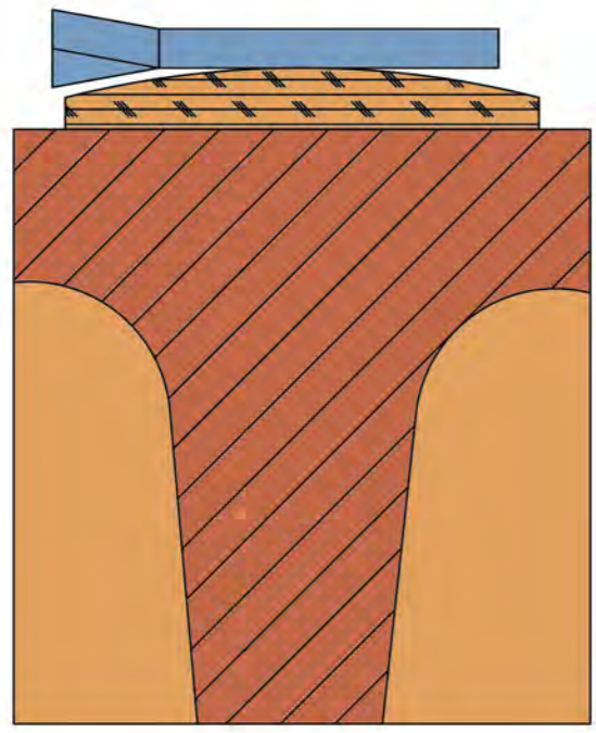
Correct position of the saw blade on the drive wheels.
